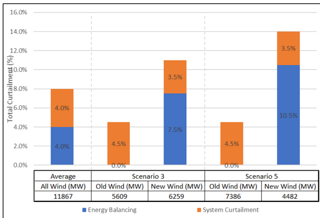
Figure 1: 2030 Wind Curtailment and Energy Balancing Estimates
