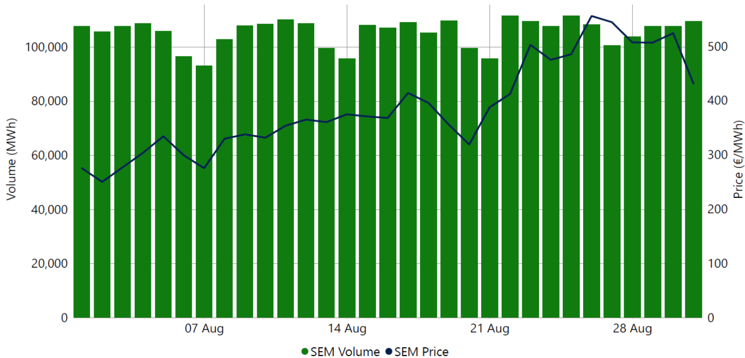
Graph 19 – DAM Daily Volume and Price
