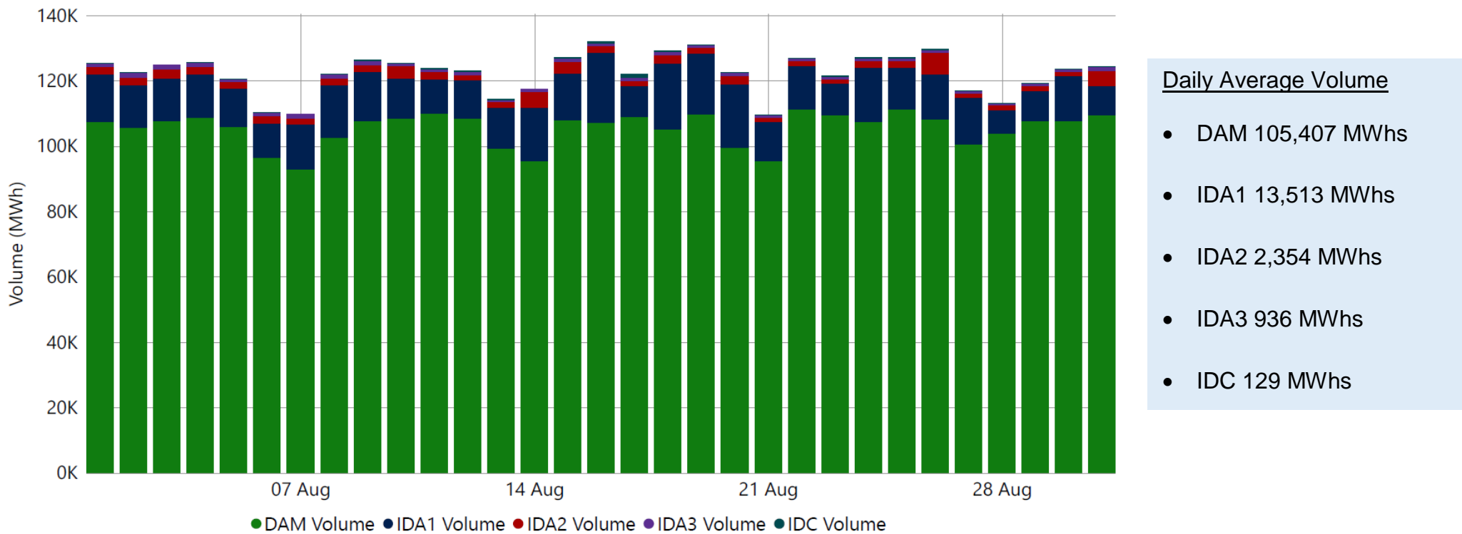
Graph 17 – Daily Ex-Ante Volumes
