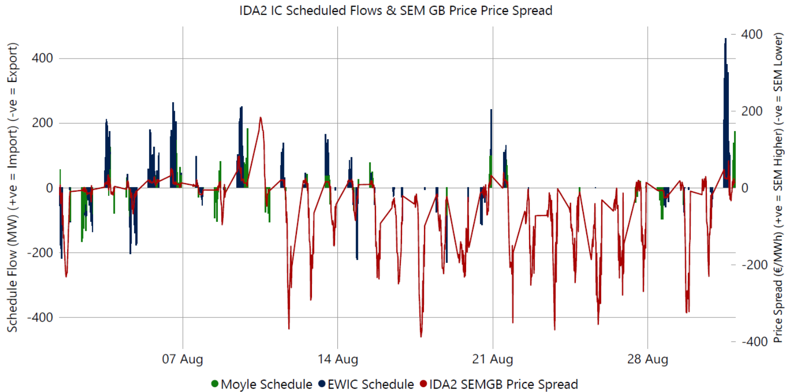
Graph 5 – IDA2 Interconnector Schedule against Price (Periods 25-48)
