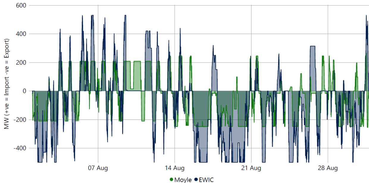
Graph 3 – Actual Interconnector Flows (15 Minute Intervals)
