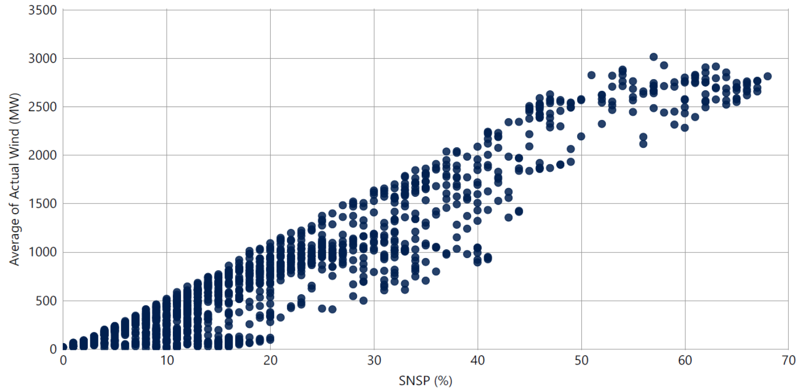
Graph 10 – SNSP against Actual Wind Generation
