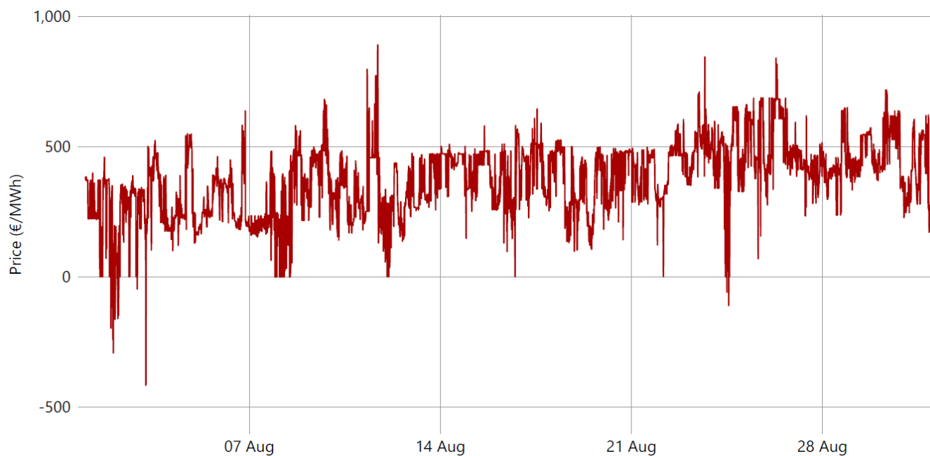
Graph 27 – 5 Minute Imbalance Pricing Period
