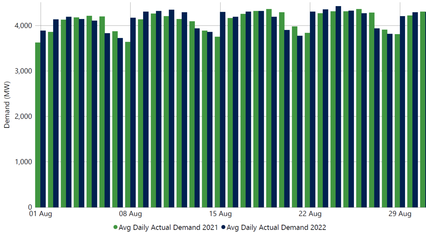
Graph 1 – Actual System Demand Daily Average 2021 against 2022
