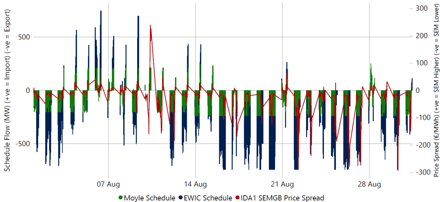
Graph 4 – IDA1 Interconnector Schedule against Price Spread (Periods 1-24)
