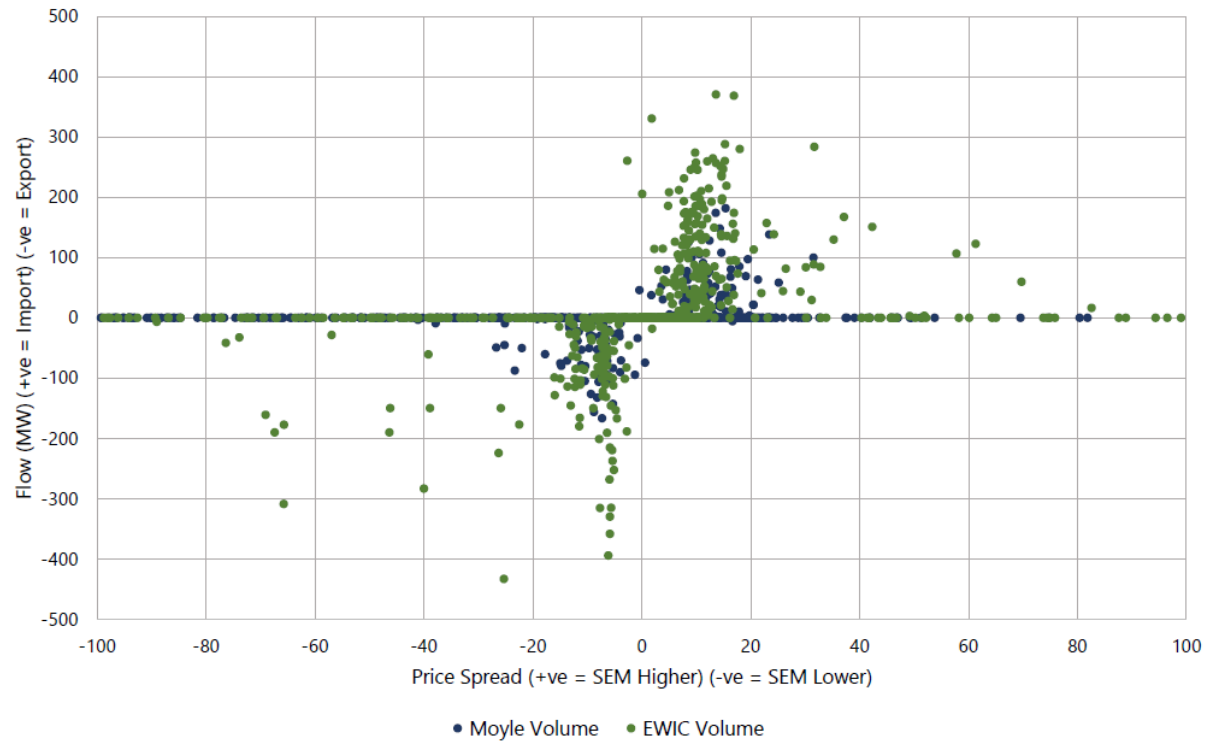
Graph 7 – IDA2 Interconnector Schedule against Price Spread (Cropped +/- €100/MWh)
