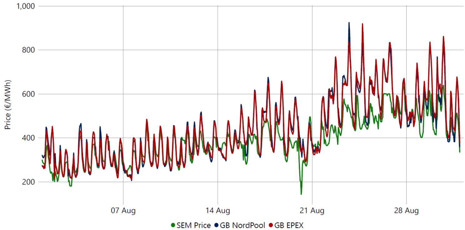
Graph 21 – DAM Hourly Prices SEM, GB EPEX & GB NordPool
