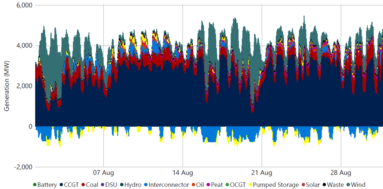
Graph 11 – Hourly Metered Generation
