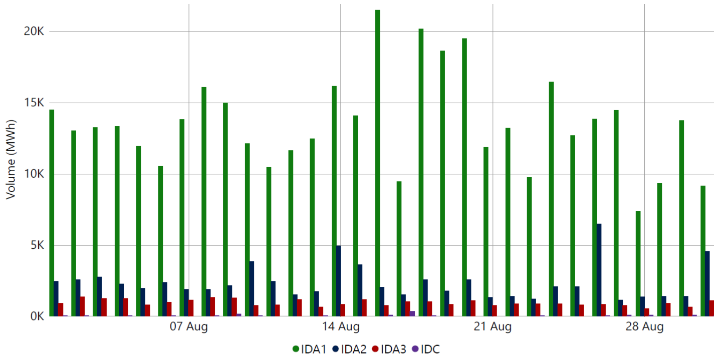
Graph 23 – Daily Total Intraday Volumes
