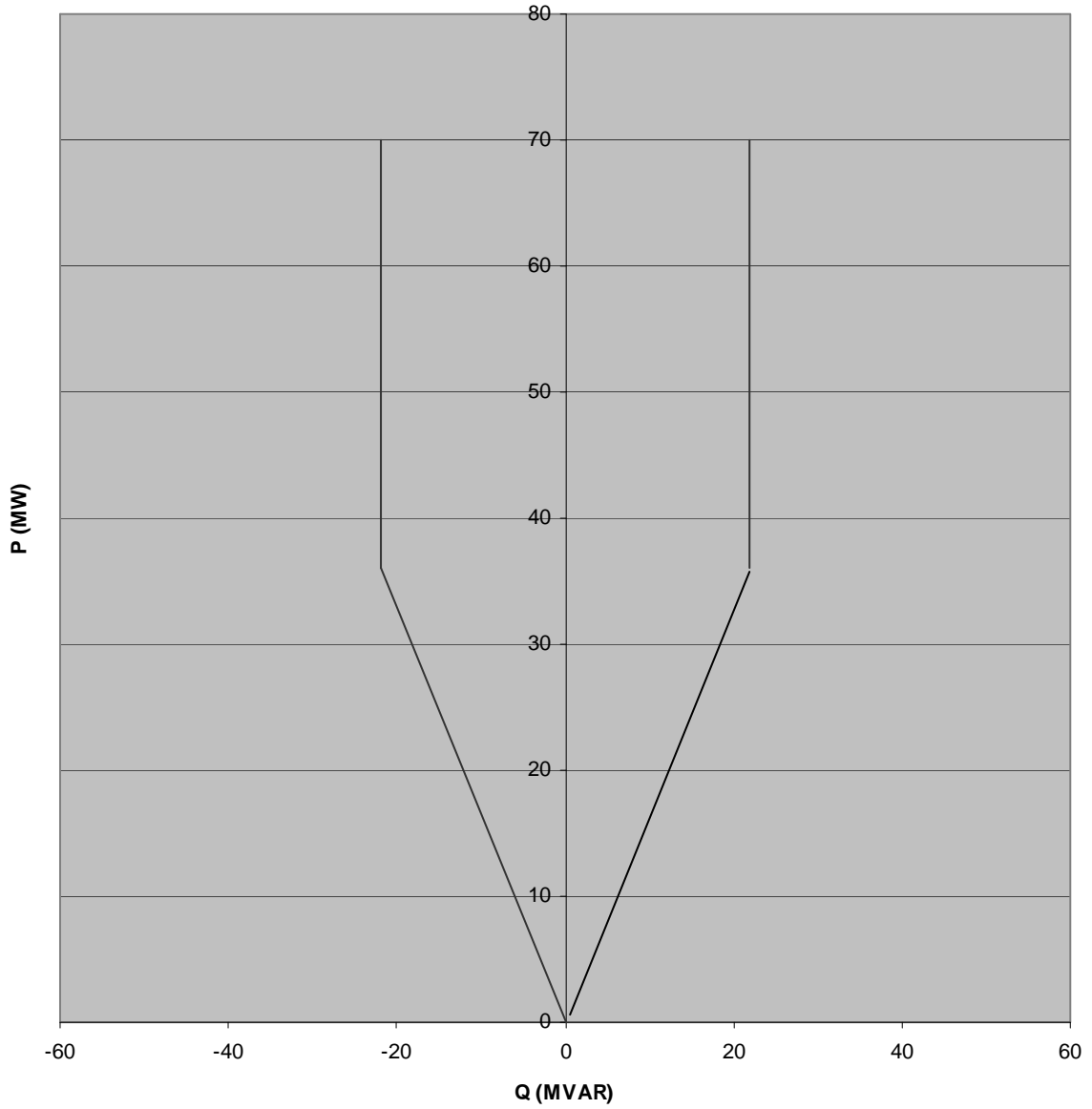
CAPABILITY CHART
