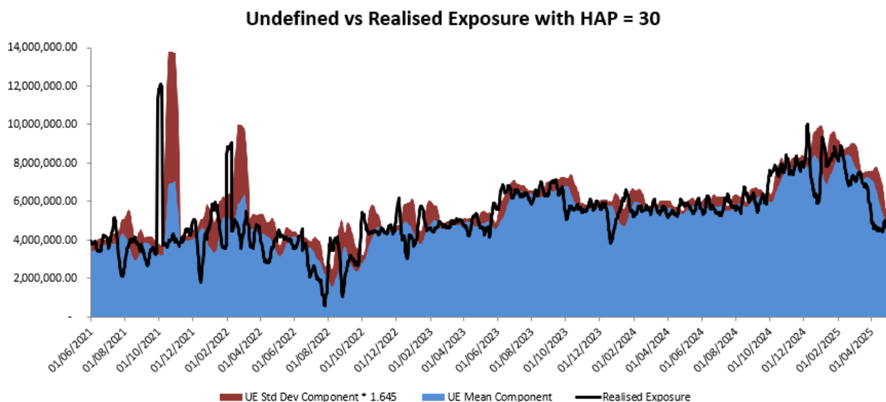
Figure 4: Estimated Undefined Exposure vs Realised Undefined Exposure with DINHAP = 30
